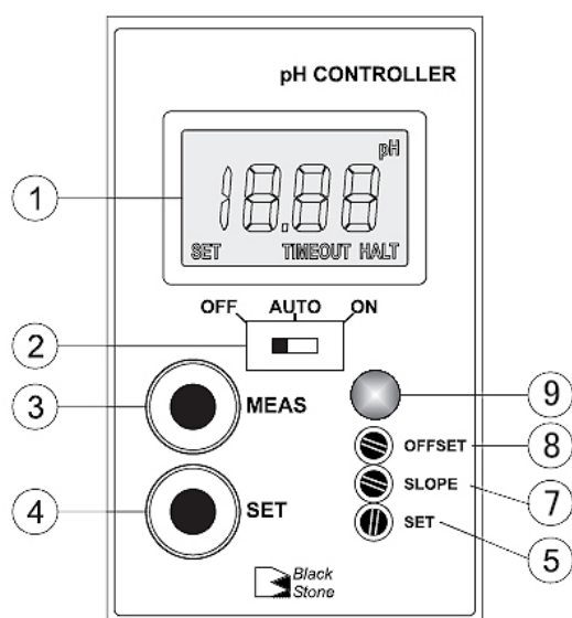
Front panel
