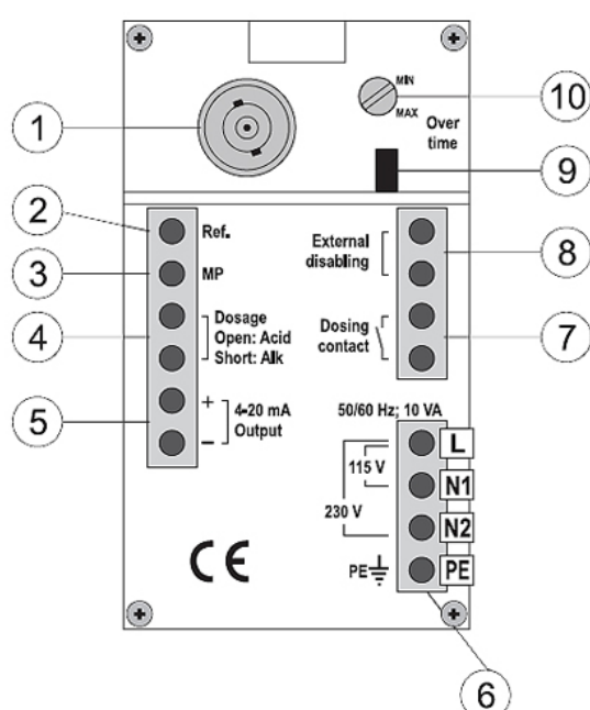
Rear panel
